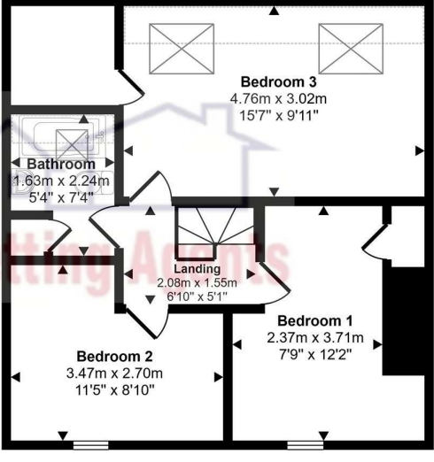
First Floor Approx 45 sq m / 488 sq ft
